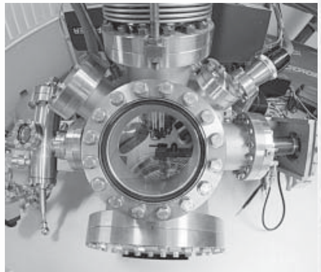
The Secondary Ion Mass Spectrometer.
